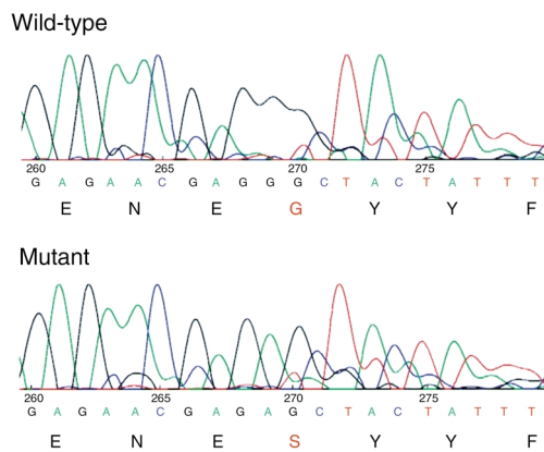
Figure 2 Mutation in the messenger RNA-coding region of the CD8 \alpha gene. Sequence of the CD8 \alpha cDNA reveals a nucleotide substitution (G→A) at position 331 (numbered from the ATG sequence initiating the coding region), leading to the replacement of a glycine by a serine at position 90.
