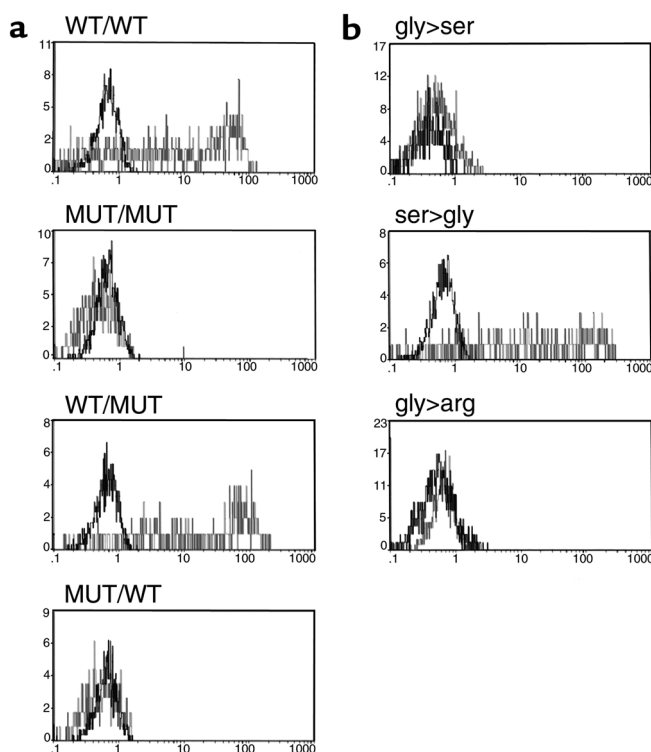
Figure 4 CD8 expression in transfected cells. COS 7 monkey kidney cells were transfected with SR \alpha 296 constructs. (a) Chimeric constructs (extracellular/transmembrane + cytoplasmic) WT/MUT and MUT/WT, wild-type CD8 \alpha (WT/WT), and mutant CD8 (MUT/MUT) were transfected. Transfected COS 7 cells were used later for immunofluorescence analysis. (b) CD8 \alpha molecules engineered by site-directed mutagenesis: CD8 gly90>ser , CD8 ser90>gly , and CD8 gly90>arg were also transfected into COS-7 cells. Gray line indicates isotype control and black line CD8 expression.
