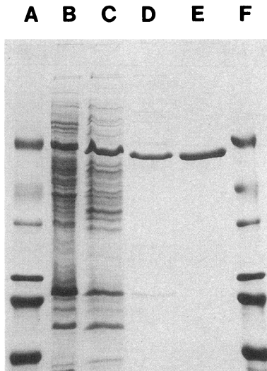
Figure 1. Purification of MCMP. MCMP was purified from L. pneumophila as described in the text. Preparations obtained after each successive stage in the purification process were examined by SDS-PAGE as follows: lane B, whole L. pneumophila ; lane C, buffer extraction; lane D, ion-exchange chromatography; and lane E, molecular sieve chromatography. Lanes A and F contain molecular weight standards (BSA, 66,000; ovalbumin, 45,000; glyceraldehyde-3-phosphate dehydrogenase, 36,000; carbonic anhydrase, 29,000; trypsinogen, 24,000; and trypsin inhibitor, 20,100).
