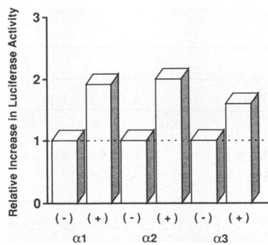
Figure 8. Relative increase in luciferase activity enhanced by 1 mM ouabain. Two types of chimeric plasmids, \alpha 1\text{LF} ( \alpha 1\text{LF} , \alpha 2\text{LF} , \alpha 3\text{LF} ) containing each \alpha isoform 5'-flanking region in the 5' end of the luciferase coding sequence, and pSV2CAT containing the simian virus 40 (SV40) enhancer and
