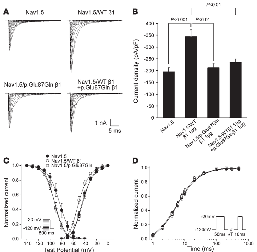
Figure 5 Electrophysiological characteristics of the p.Glu87Gln mutant. (A) Representative traces of sodium current. (B) Current density at -30 mV for Nav1.5 alone ( n = 13 ), Nav1.5 coexpressed with WT \beta 1 ( n = 17 ), Nav1.5 coexpressed with p.Glu87Gln \beta 1 ( n = 18 ), and Nav1.5 coexpressed with WT \beta 1 plus p.Glu87Gln \beta 1 ( n = 15 ). (C) Voltage dependence of activation and inactivation. Filled circles, open circles, and squares indicate Nav1.5 alone, Nav1.5 coexpressed with WT \beta 1 , and Nav1.5 coexpressed with p.Glu87Gln \beta 1 , respectively. (D) Recovery from inactivation. Biophysical properties are provided in Table 2.
