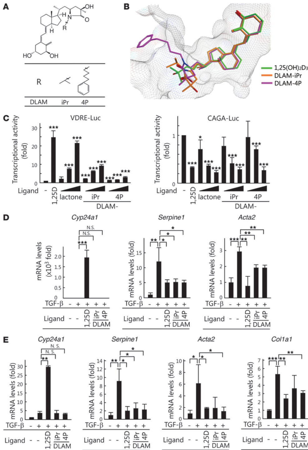
Figure 6 DLAM derivatives that suppress TGF- \beta -dependent transcription without VDR transactivation. (A) DLAM derivatives, DLAM-iPr and DLAM-4P, used in this study. (B) Binding of DLAM-iPr and DLAM-4P to agonistic VDR. The DLAM derivatives were docked into the ligand-binding pocket in the VDR-LBD complexed with 1,25(OH) _2 D _3 (PDB: 1DB1) using MOE. The ligand-binding pocket of VDR-LBD- \Delta H12 is represented as a mesh model. (C) Dose responses of DLAM-iPr and DLAM-4P. Plasmids encoding ALK5 TD and VDR were transfected with reporter plasmids VDRE-Luc and CAGA-Luc into HEK293 cells. After culturing transfected cells with or without 1,25(OH) _2 D _3 (10 nM), 1,25-lactone (0.01, 0.1, or 1 \mu M), or DLAM derivatives (0.01, 0.1, or 1 \mu M) for 24 hours, cell extracts were analyzed in luciferase assays. (D) TCMK-1 cells were cultured in the presence or absence of 5 ng/ml TGF- \beta and 10 nM 1,25(OH) _2 D _3 , 1 \mu M DLAM-iPr, or 1 \mu M DLAM-4P. Cyp24a1 , Serpine1 , and Acta2 mRNA levels were determined using qPCR. (E) Kidney fibroblasts were isolated and cultured in the presence or absence of 5 ng/ml TGF- \beta and 10 nM 1,25(OH) _2 D _3 , 1 \mu M DLAM-iPr, or 1 \mu M DLAM-4P for 8 hours, and Cyp24a1 , Serpine1 , Acta2 , and Col1a1 mRNA levels were determined using qPCR. * P < 0.05; ** P < 0.01; *** P < 0.001.
