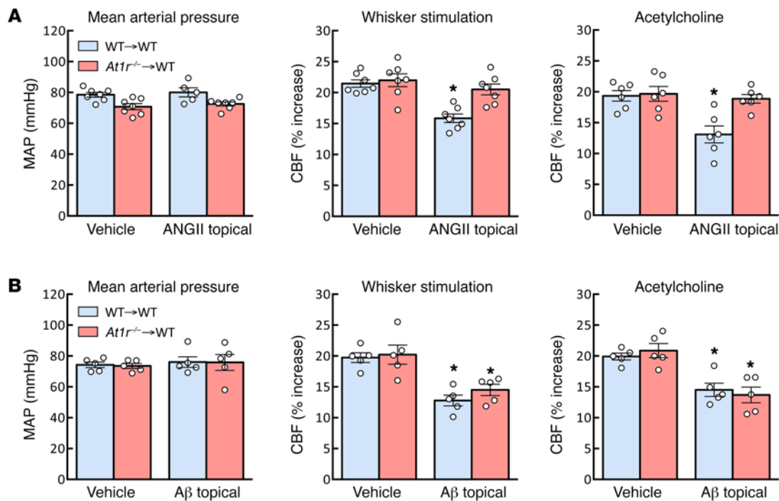
Figure 6. At1r deletion in PVMs rescues the neurovascular dysfunction induced by topical neocortical application of ANGII but not amyloid-β. (A) At1r -/- →WT chimeras are protected from the cerebrovascular effects induced by topical neocortical application of ANGII. * P < 0.05 vs. WT→WT-Veh and At1r -/- →WT-Veh; n = 5–7 per group (2-way repeated-measures ANOVA and Bonferroni's test). (B) The attenuation of the CBF responses induced by topical application of amyloid-β (Aβ), an effect not dependent on AT1Rs, is not affected. This finding attests to the specificity of the effect of PVM At1r deletion on the cerebrovascular dysfunction induced by ANGII. * P < 0.05 vs. WT→WT-Veh and At1r -/- →WT-Veh (2-way repeated-measures ANOVA and Bonferroni's test).
