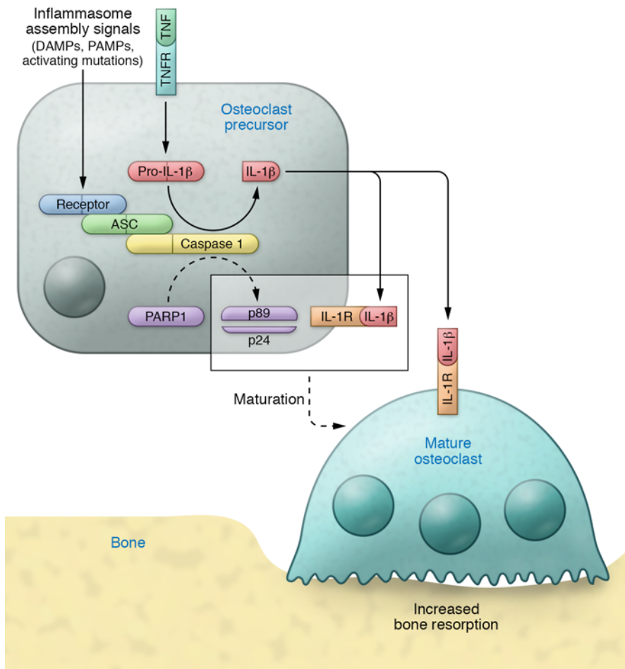
Figure 2. The inflammasomes in osteolysis. Cytokines such as TNF induce the expression of pro-IL-1 \beta , which lacks the signal peptide for secretion. Recognition of damage- or pathogen-associated molecular patterns (DAMPs or PAMPs) by the receptor/sensor component of the inflammasome (e.g., NLRP3, NLRC4), or activating mutations of some of these receptors, leads to the assembly of the inflammasome, a protein complex containing the receptor, apoptosis-associated speck-like protein containing a CARD (ASC) and caspase 1. Once assembled, this active complex cleaves pro-IL-1 \beta into active IL-1 \beta and triggers cascades that lead to PARP1 cleavage into p89 and p24 fragments. In precursors sensing DAMPs or PAMPs, cleaved PARP1 and autocrine effects of IL-1 \beta , acting through IL-1R, promote maturation of osteoclasts into bone-resorbing cells. Secreted IL-1 \beta can also act in a paracrine manner to increase bone resorption by nearby osteoclasts. Dashed arrows indicate multiple steps.
