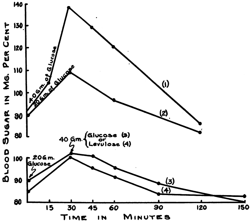
FIG. 6. CURVES ILLUSTRATING THE EFFECT OF ARTIFICIAL ELEVATION OF THE BLOOD SUGAR LEVEL PRIOR TO THE LEVULOSE OF GLUCOSE TOLERANCE TESTS
