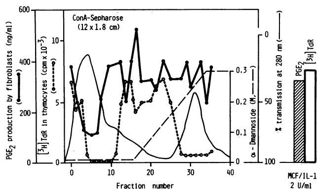
Figure 4. Fresh urine (30 ml from H.P.) was precipitated between 40 and 80% (NH 4 ) 2 SO 4 . The precipitate 2.85 mg was chromatographed on Con A-Sepharose in 0.05 M Tris-HCl (pH 7.4), 0.2 M NaCl, 1 mM MgCl 2 , 1 mM CaCl 2 . An elution gradient was performed with 0.3 M \alpha -D-methylmannoside. Eluted fraction (5 ml/fraction) were diluted 1:40 and assayed for PGE 2 -stimulating activity on dermal fibroblasts ( \bullet ) and for urine thymocyte proliferation. Bars represent the MCF/IL-1 stimulation alone for PGE 2 ( \blacksquare ) and thymocyte proliferation ( \square ).
